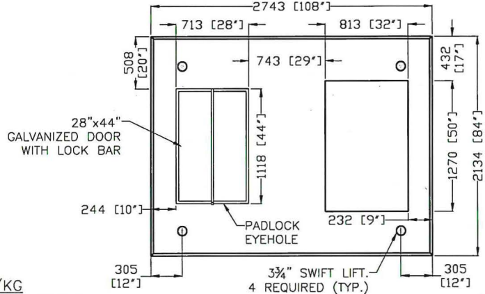
LID FRONT VIEW
