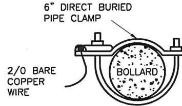
GROUND WIRE CONNECTION DETAIL FOR POURED IN PLACE BOLLARD
