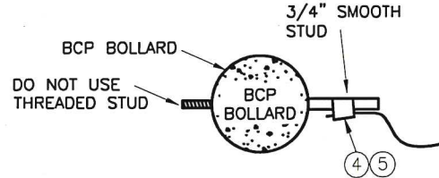
GROUND WIRE CONNECTION DETAIL FOR BROOKLIN BCP BOLLARD
