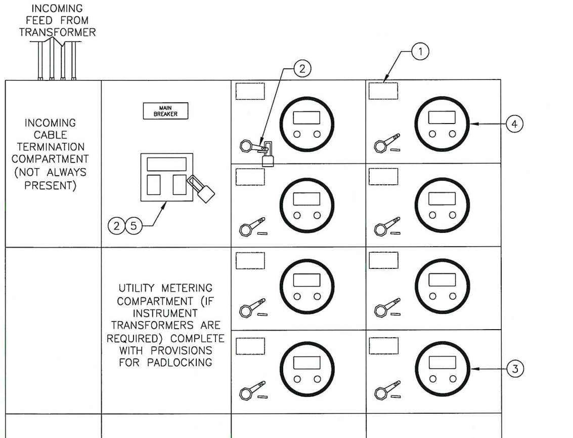
FINISHED FLOOR ELEVATION
